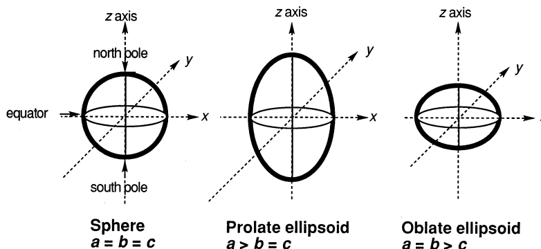
Fig. 5. A sphere, prolate ellipsoid, and oblate ellipsoid as examples of momental ellipsoids indicating the positions of the poles and the equator.
