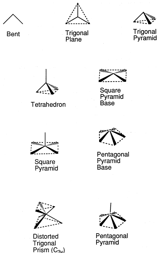
Fig. 11. Possible (i.e., symmetry allowed) shapes of early transition metal complexes using a six-orbital sd^5 manifold.
